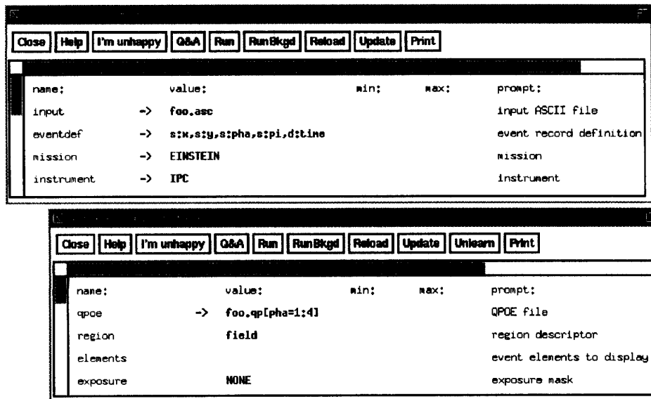
Figure 2: ASSIST's parameter editors for controlling software modules
