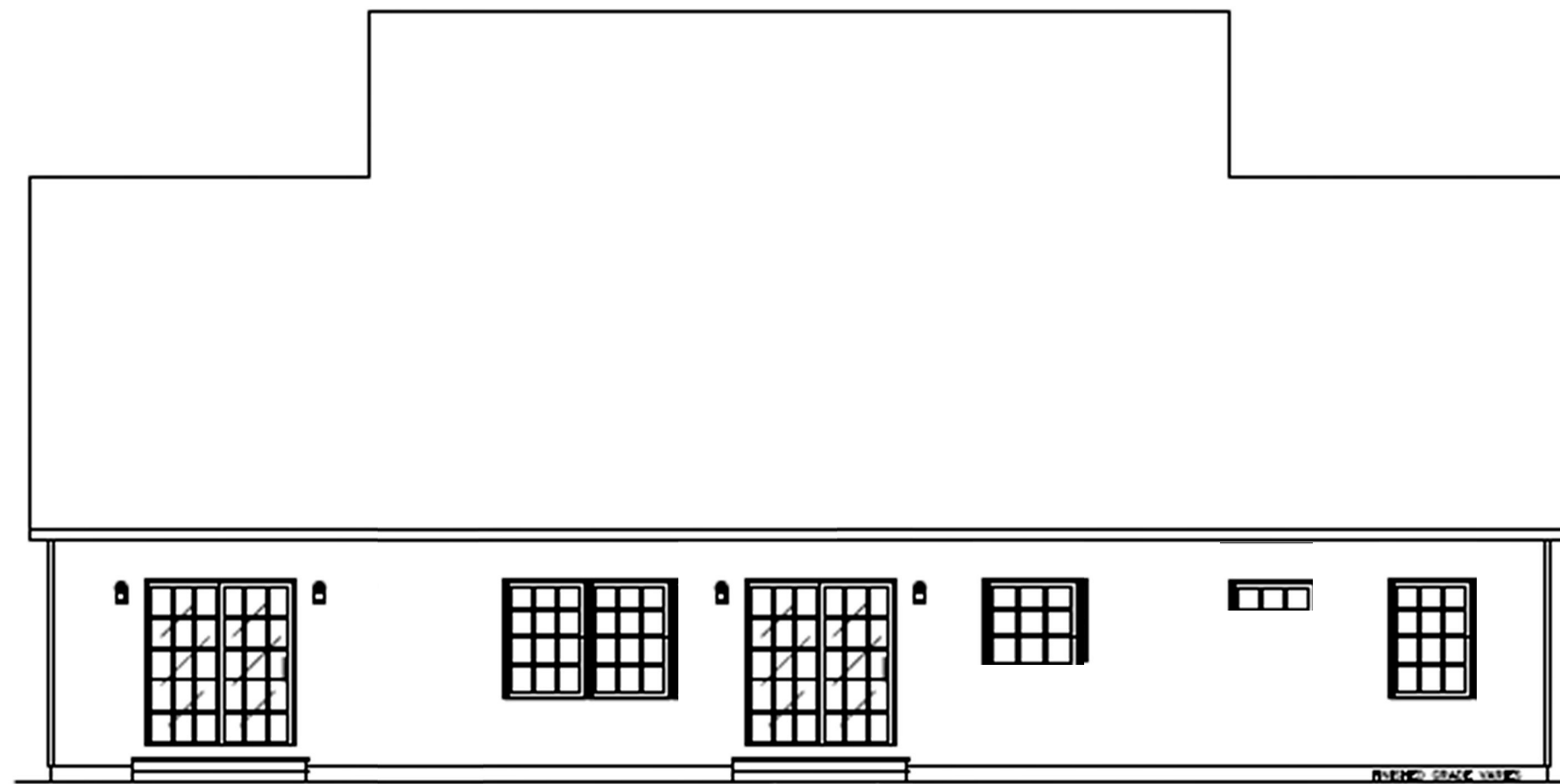
REAR ELEVATION
