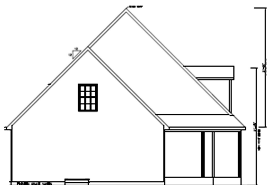
LEFT ELEVATION
