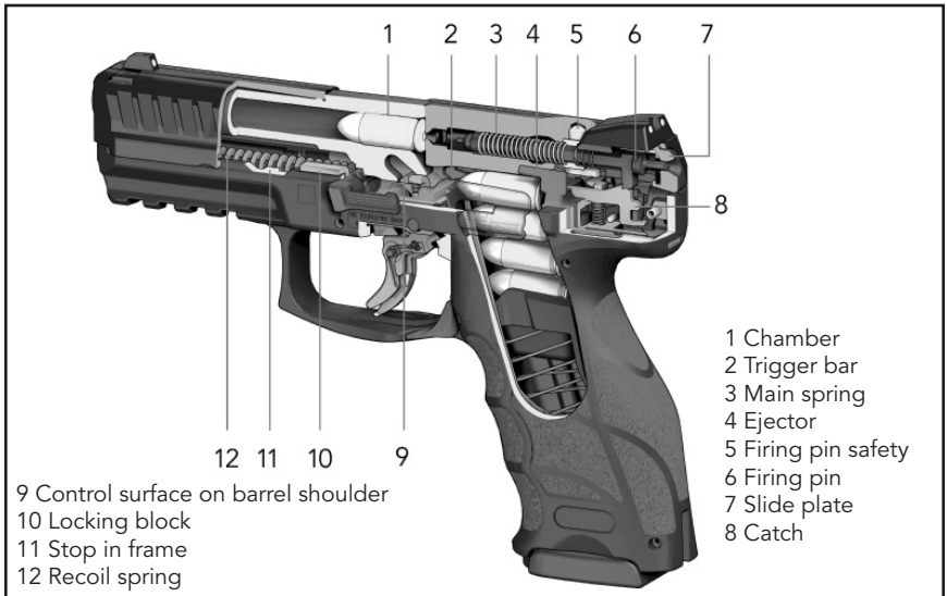
Figure 3 — VP9 Cutaway View
