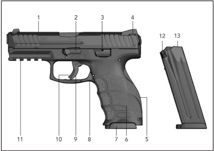
Figure 2 — VP9 (right side view)
