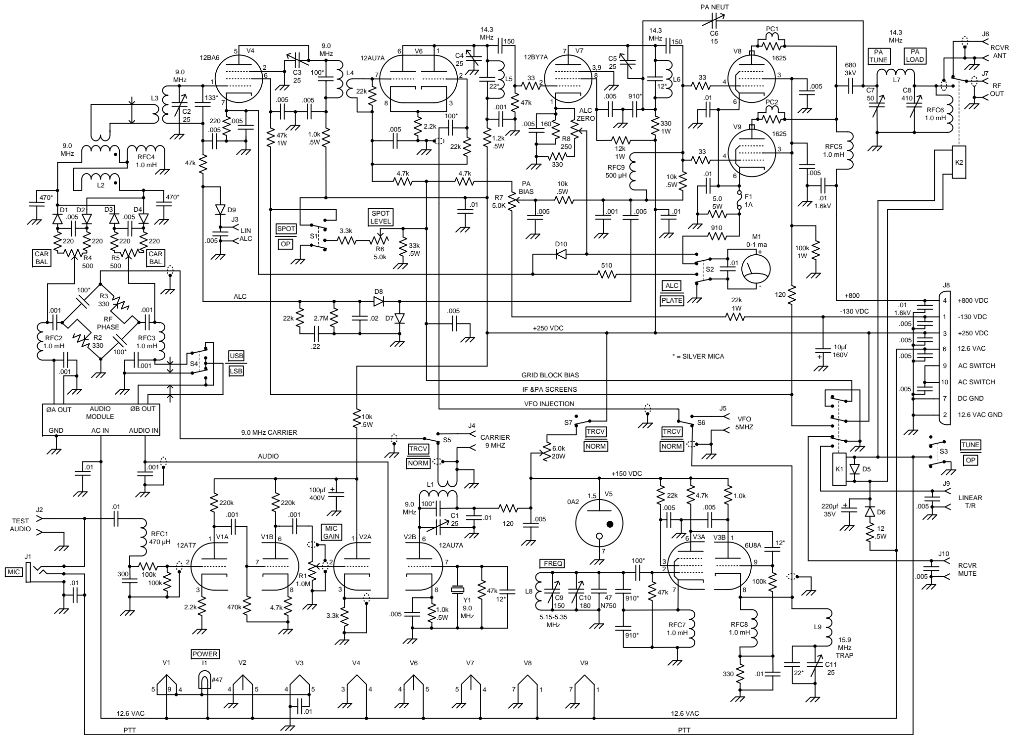
TRANSMITTER SCHEMATIC
