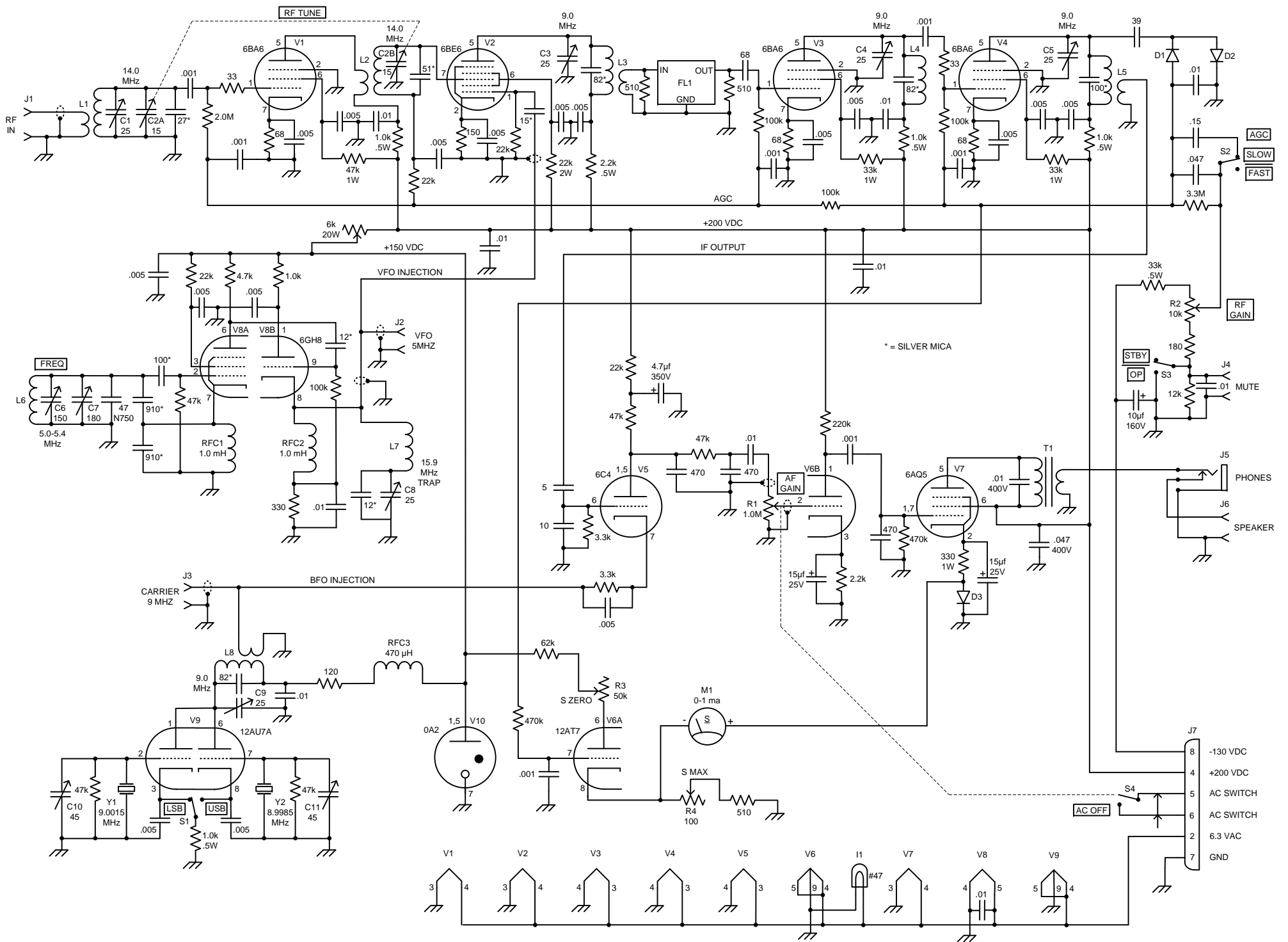
RECEIVER SCHEMATIC
