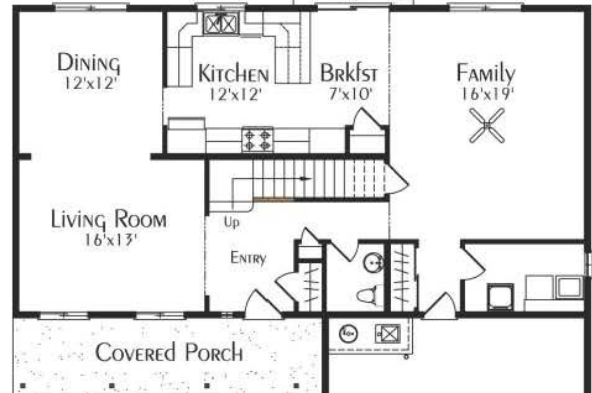
Main Floor SqFt. = 1248 9' Tall Walls GARAGE SqFt. = 573
