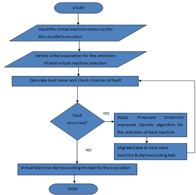
Fig.1: Flowchart of Proposed Enhanced Improved Genetic Algorithm
