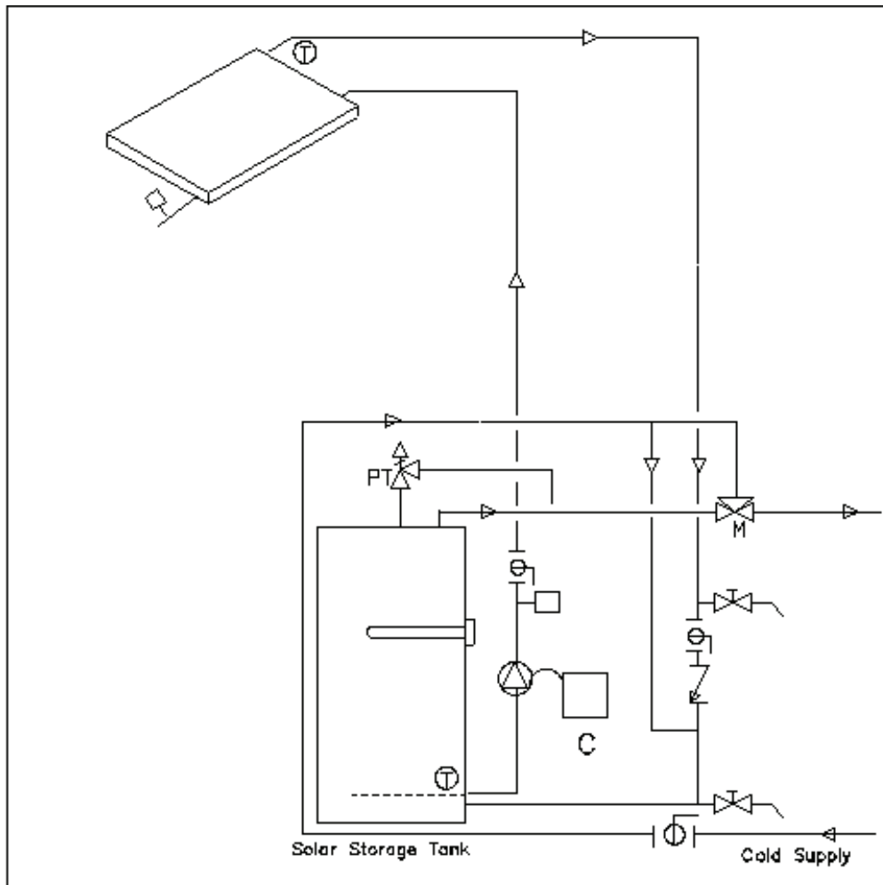
OG-300 System Reference:2008001A SVG Diagram Display
