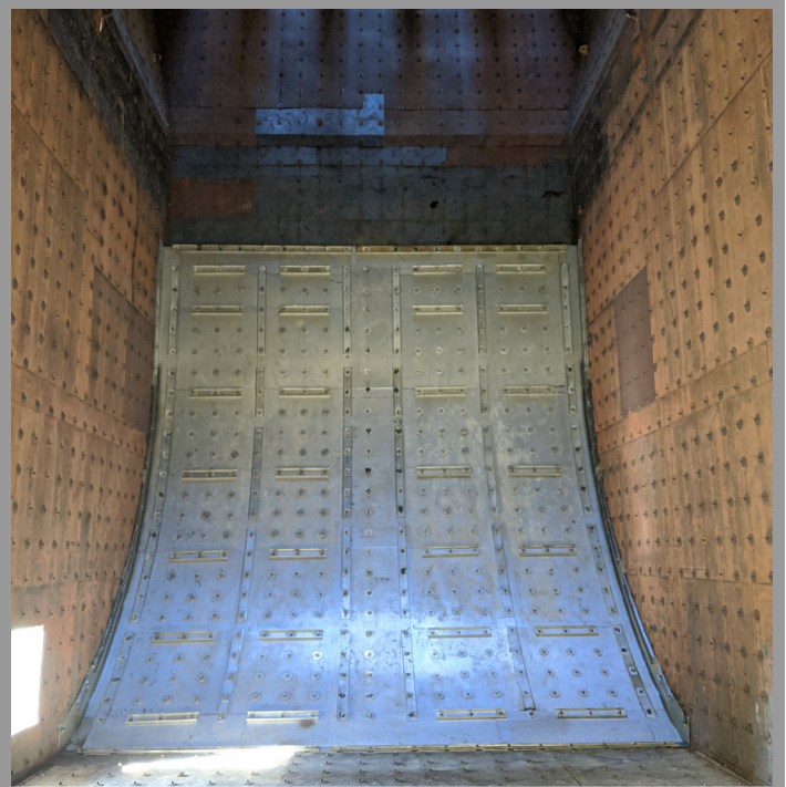
Curved Floating Liner System
