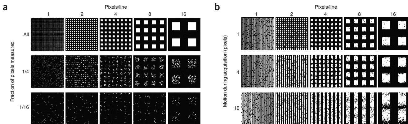
Figure 1 | Factors influencing spatial resolution in live-cell PALM. (a) Resolution versus the density of localized molecules, represented here as pixels in a test pattern. Features are imaged at progressively lower signal-to-noise ratio as the molecular density decreases and become unresolvable when the mean molecular separation approaches the feature size. As more time is required to localize more molecules, this illustration implies a fundamental trade-off between spatial and temporal resolution in PALM. (b) Resolution versus feature motion. The serial, stochastic acquisition process in PALM leads to another such trade-off: the resolution limit for dynamically evolving features is comparable to the product of the feature velocity and the frame acquisition time.
