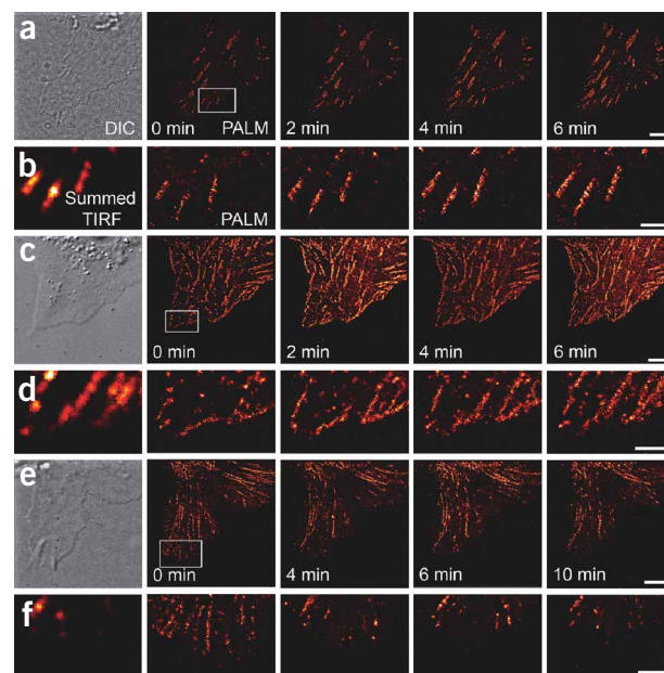
Figure 4 | Paxillin flow to and from ACs. ( a–f ) Selected live-cell PALM images ( a,c,e ; scale bars, 5 \mu m) and higher-magnification views ( b,d,f ; scale bars, 2 \mu m) of boxed regions of tdEos-paxillin distributions in several cells. DIC and summed TIRF microscopy images are shown at left. The NIH 3T3 cell in a,b and Supplementary Video 4 showed inward AC motion (upward, toward the cell center) but no new AC formation at the cell periphery, similar to the adhesions we observed in 12 additional cells (data not shown). In contrast, the CHO cell in c,d and Supplementary Video 5 displayed inward motion and a constant replenishment of paxillin molecules at the cell edge, typical of the adhesions in 8 additional cells we observed (data not shown). The NIH 3T3 cell in e,f retracted with a resulting dissolution of ACs ( Supplementary Video 6 ), similar to the dissolving ACs we observed in 8 additional cells (data not shown). Indicated times are final time points of each 30 s acquisition ( a,b ) or 60 s acquisition ( c–f ), with the first time in the image series set to 0 s.
