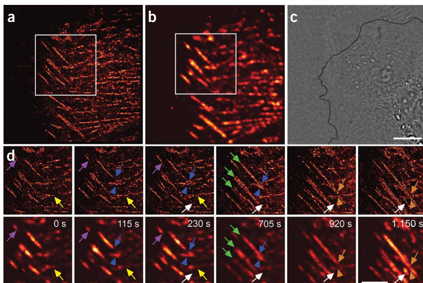
Figure 3 | Live-cell PALM allows extended observations at high resolution and over a wide range of molecular density. ( a–c ) PALM ( a ), summed TIRF ( b ; Supplementary Video 3 ) and DIC ( c ) images of a CHO cell expressing tdEos-paxillin, imaged for >20 min. ( d ) Higher-magnification views of boxed regions in a (top row) and b (bottom row) showing predominantly horizontal and stationary adhesions (yellow arrows) and diagonal inwardly moving adhesions (purple arrows). Intersecting adhesions either interacted weakly (orange arrows and arrowheads) or the moving AC bends the stationary AC (blue arrows and arrowheads). Features that appeared homogeneous in summed TIRF microscopy were revealed at their true size with substantially greater internal detail by PALM (green arrows). PALM also revealed nascent adhesions initially not seen by summed TIRF microscopy that arose in the cell interior (white arrows). Indicated times are final time points of each 60-s acquisition, with the first time in the image series set to 0 s. Scale bars, 5 \mu m.
