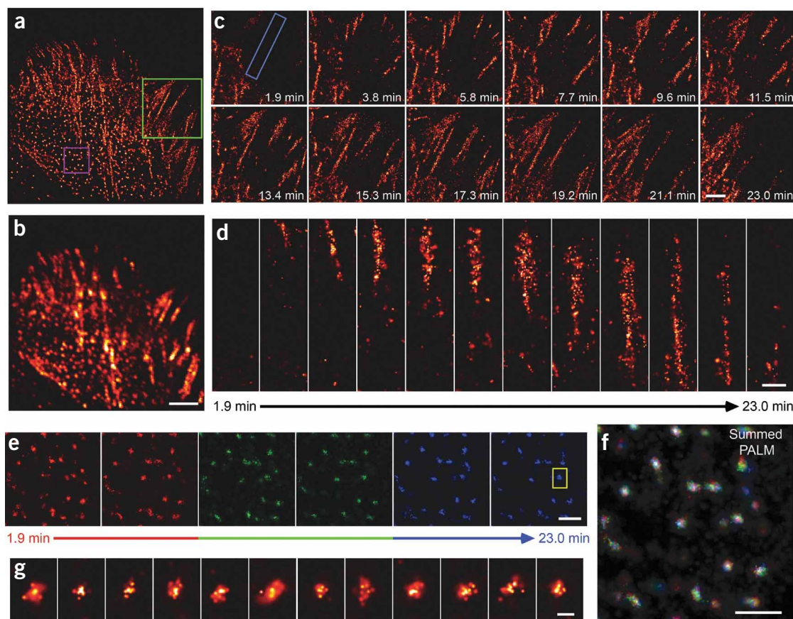
Figure 5 | A diversity of AC dynamics in a single cell. (a,b) PALM (a) and summed TIRF microscopy (b) images of a CHO cell expressing tdEos-paxillin from a 23-min time series (Supplementary Video 7). Scale bar, 5 \mu\text{m} . (c) Higher magnification of the green-boxed region in a to illustrate AC initiation and elongation. Note the established ACs at lower left in addition to paxillin molecules that are less well organized in regions at upper right. Scale bar, 3 \mu\text{m} . (d) Higher magnification of a single AC (boxed region in c) to visualize molecular organization during the elongation process. Scale bar, 0.5 \mu\text{m} . (e–g) The motion of subdiffraction ACs (magenta box in a) is highlighted in the time series. The initial, middle and late frames in e were colored red, green and blue, and then added to create the time-summed pseudocolor image in f. Scale bars, 0.5 \mu\text{m} . The mostly white central cores in f, the higher magnification view of the single AC (g; close-up of boxed region in e) and Supplementary Video 8 suggest the central portions of ACs are constrained to regions that are small compared to AC diameters. Indicated times are final time points of each 55 s acquisition, with the first time in the image series set to 0 s. Scale bar, 0.05 \mu\text{m} .
