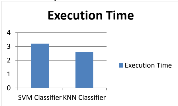
Fig. 3: Execution Time
