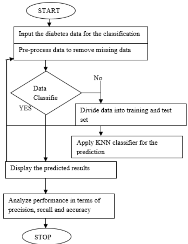
Fig.1: Proposed Methodology
