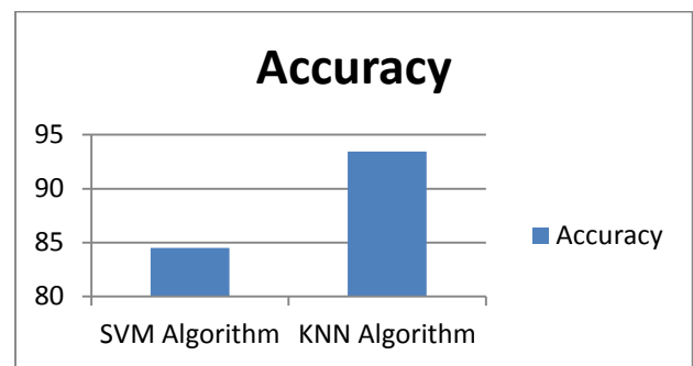
Fig. 2: Accuracy Comparison
