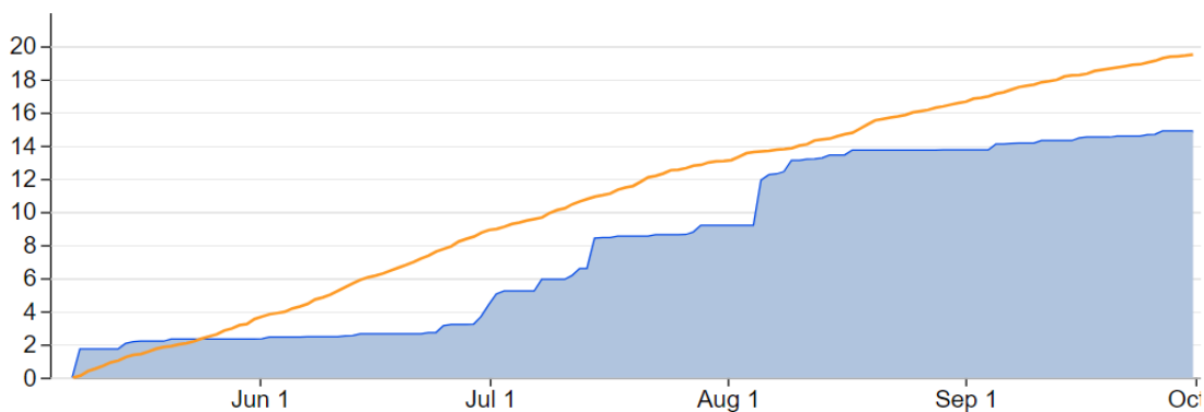
Accumulated Precipitation
