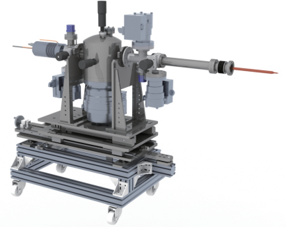
BL1100s (He MONO)
