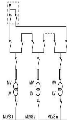
b) Open ring, 1 MV substation:
