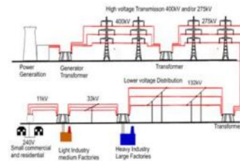
POWER GENERATION&TRANSMISSION
