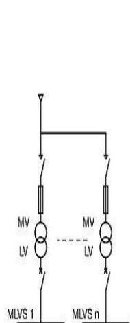
a) Single feeder:
