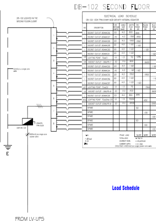
Load Schedule
