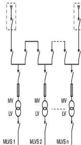
c) Open ring, 2 MV substations:
