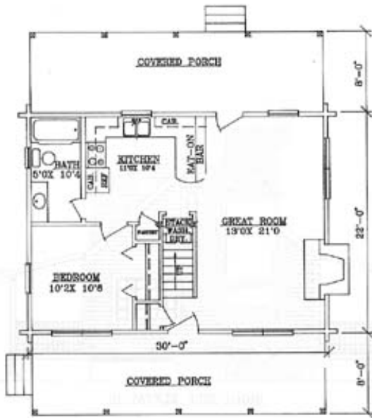
FIRST FLOOR PLAN 660 SQ. FT
