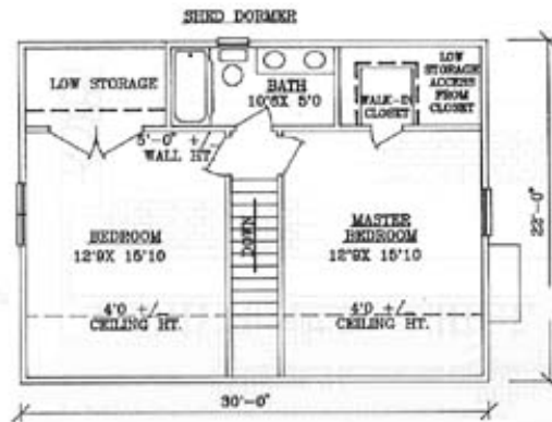
SECOND FLOOR PLAN 660 SQ. FT
