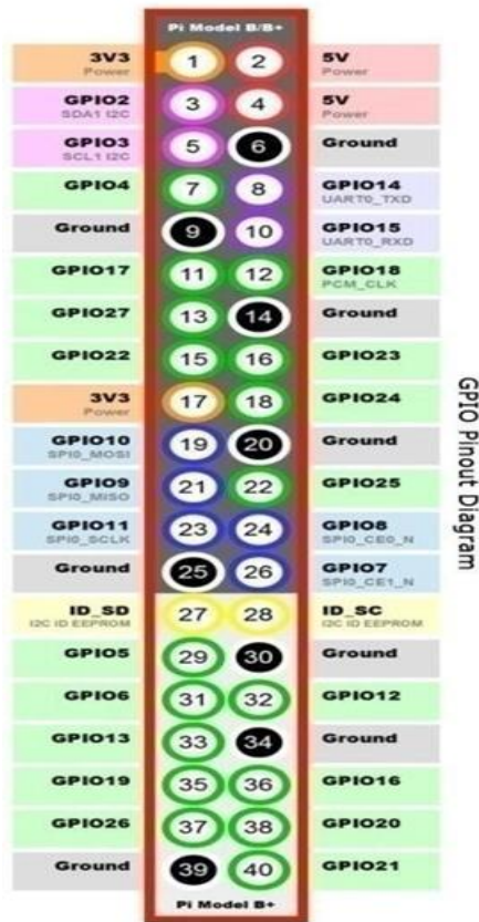
Fig.3: Raspberry Pi 3 Pin Configuration
