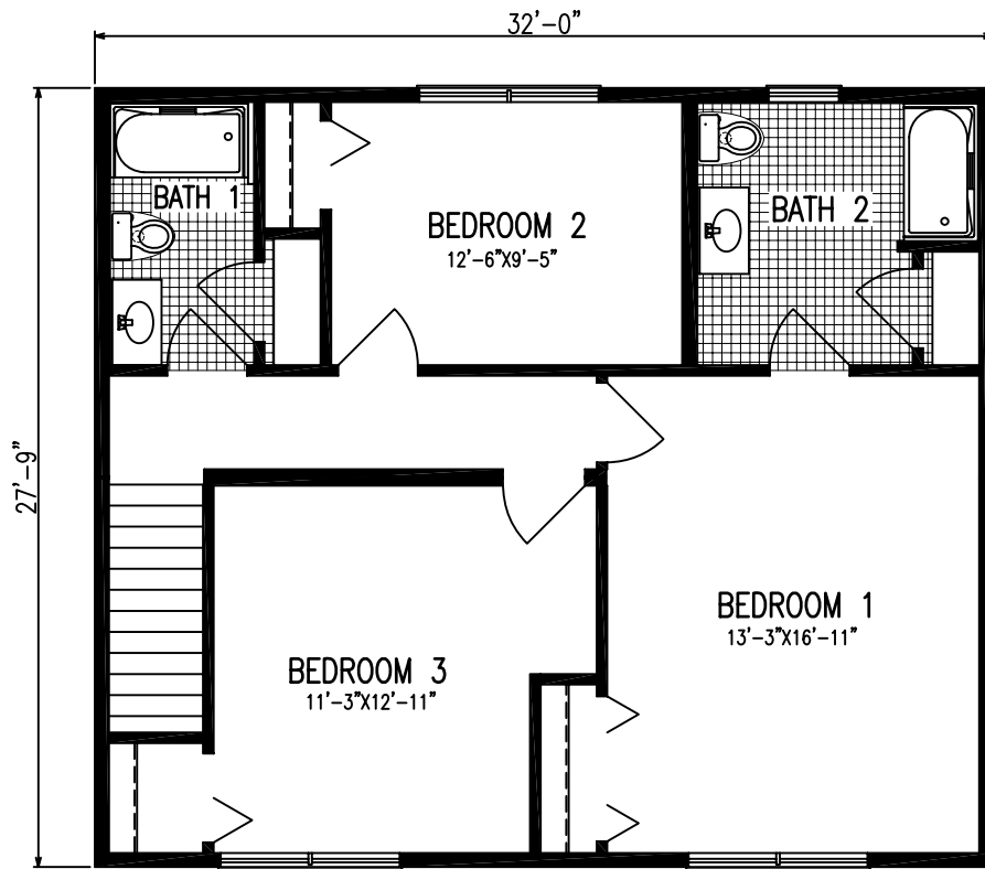
2ND FLOOR- 896 SQ FT
