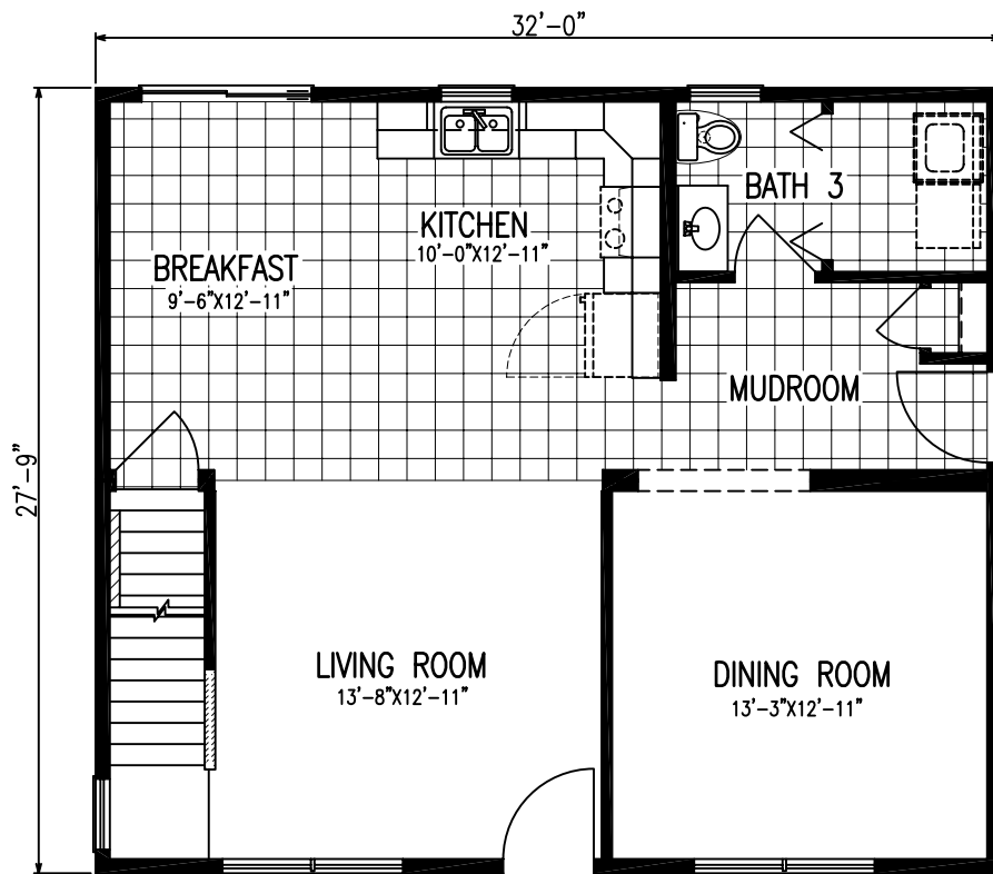
1ST FLOOR- 896 SQ FT
