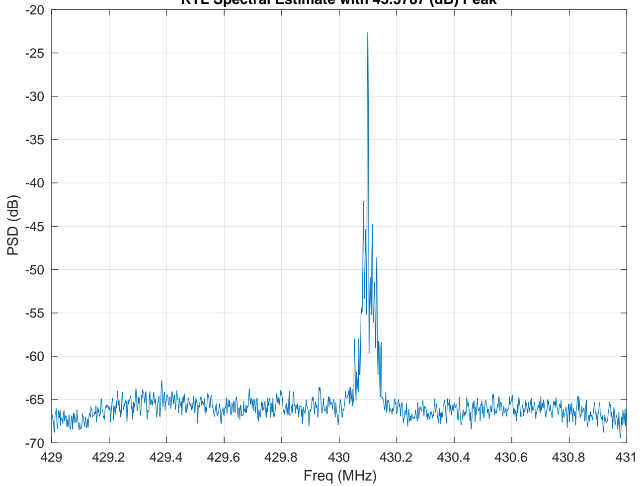
RTL Spectral Estimate with 43.3787 (dB) Peak
