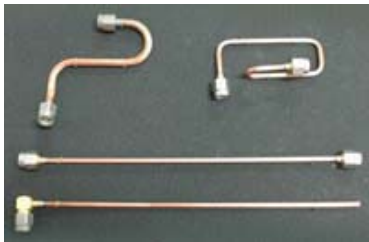
SEMI RIGID CABLE ASSEMBLY
