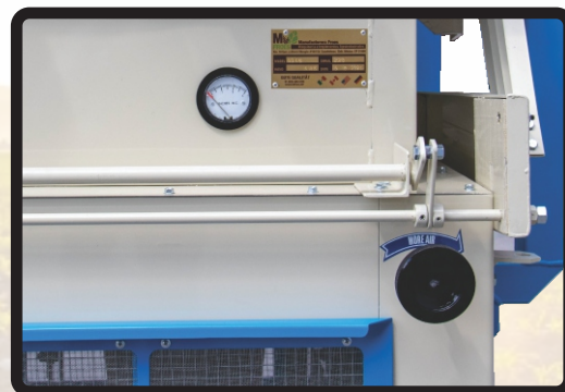
Air gauge & Air flow adjustment wheel
