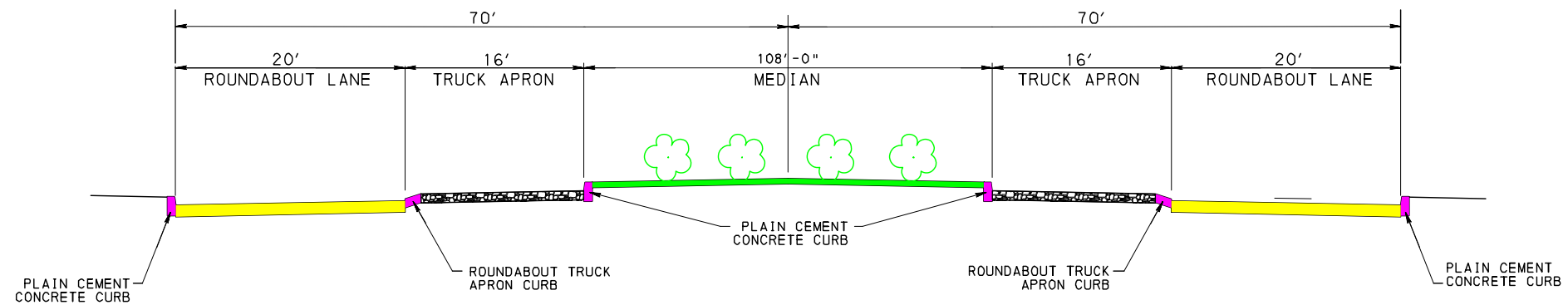
ROUNDABOUT TYPICAL
