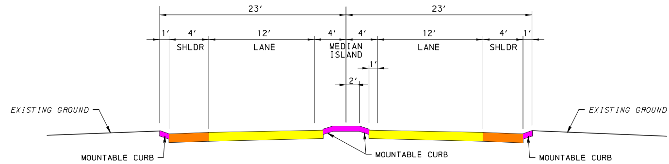
SR 0041 TYPICAL
