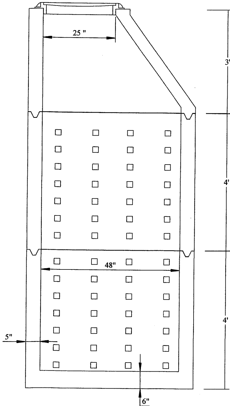
Type "B" Drywell
