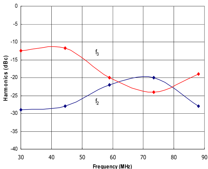
Figure 3: RFPS30-88-50 Typical f 2 and f 3 @ P out = 50W.
