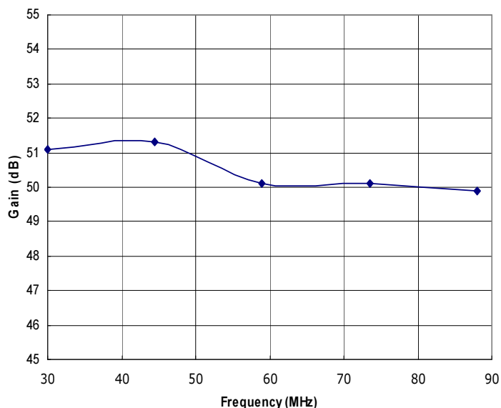
Figure 1: RFPS30-88-50 Typical Gain @ P out = 50W.
