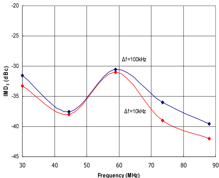
Figure 2: RFPS30-88-50 Typical IMD 3 @ 50W PEP, Δf=10kHz and Δf=100kHz. For improved linearity, see our RFPS30-88-25 Class A amp.
