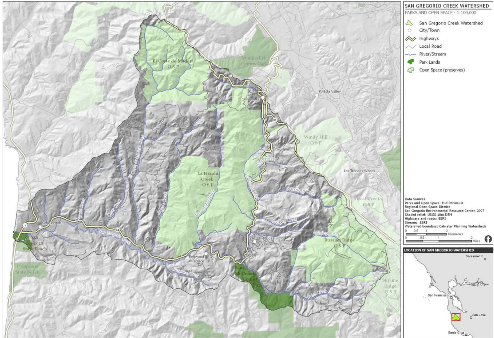
Figure 2-2. Park lands and open space preserves in the San Gregorio Creek watershed.
