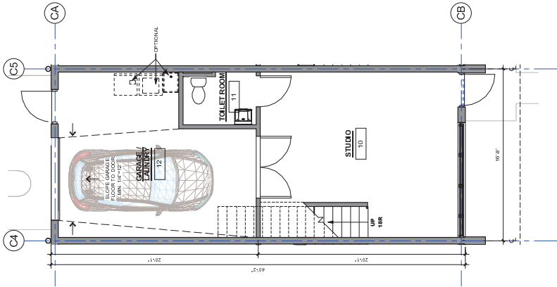
10 - Typical Townhouse - Studio Level - M 1/8" = 1'-0"
