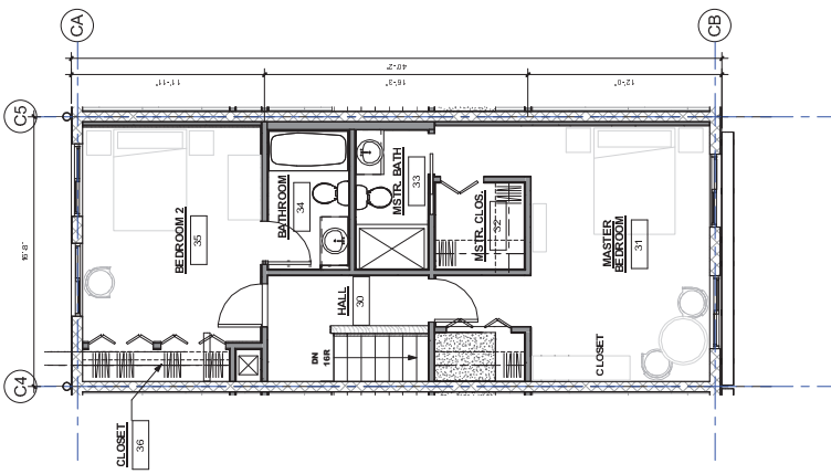
30 - Typical Townhouse - Sleeping Level - M 1/8" = 1'-0"
