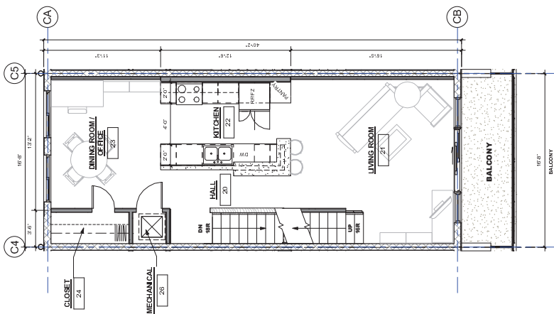
20 - Typical Townhouse - Living Level - M 1/8" = 1'-0"
