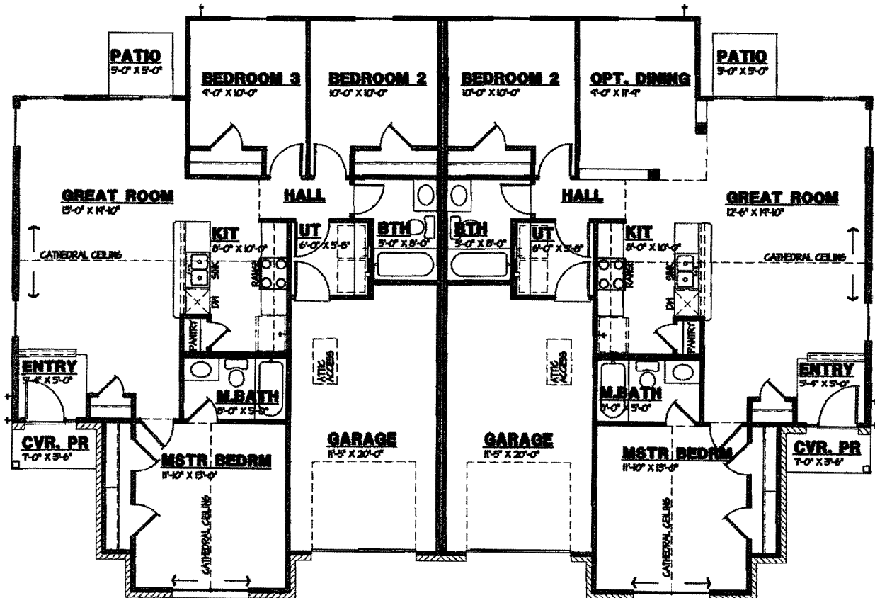
1060 FLOOR PLAN
