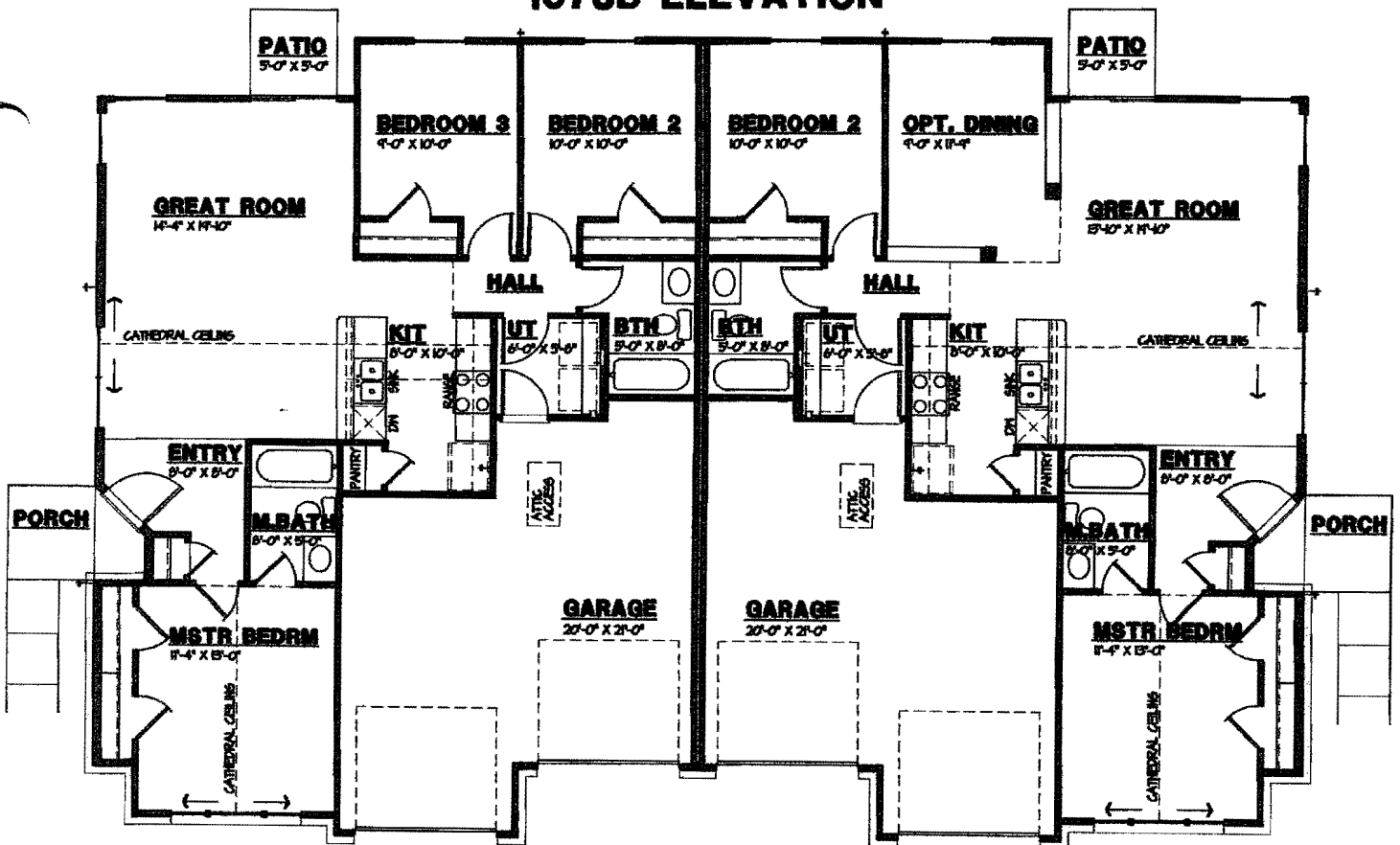
1073 FLOOR PLAN
