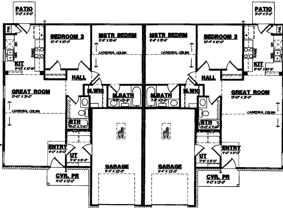
905 FLOOR PLAN
