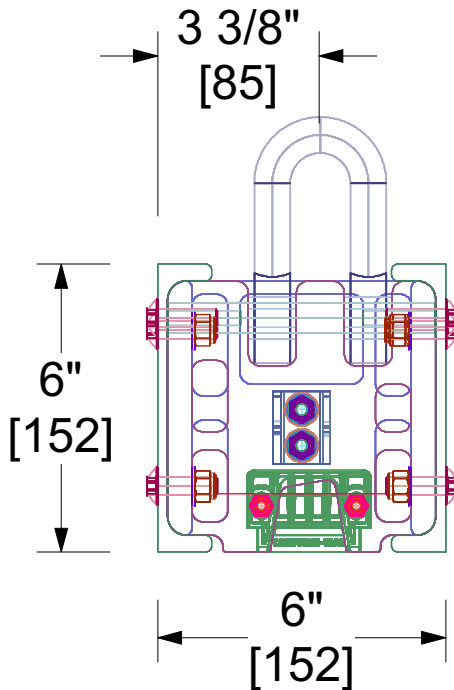
3 Right View 3" = 1'0"
