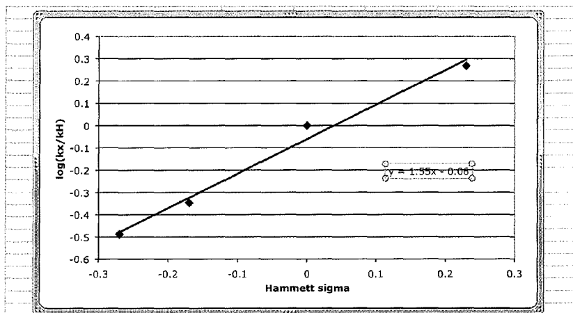
Linear free energy correlation between rate of H-Lys(DNP)-OH release where, R^2 = -(CH_2)_3C\equiv CH at 25°C from compounds of Figure 5 and the Hammett \sigma_p ; left to right, R^1 = -OMe, -CH_3, -H, -Cl
