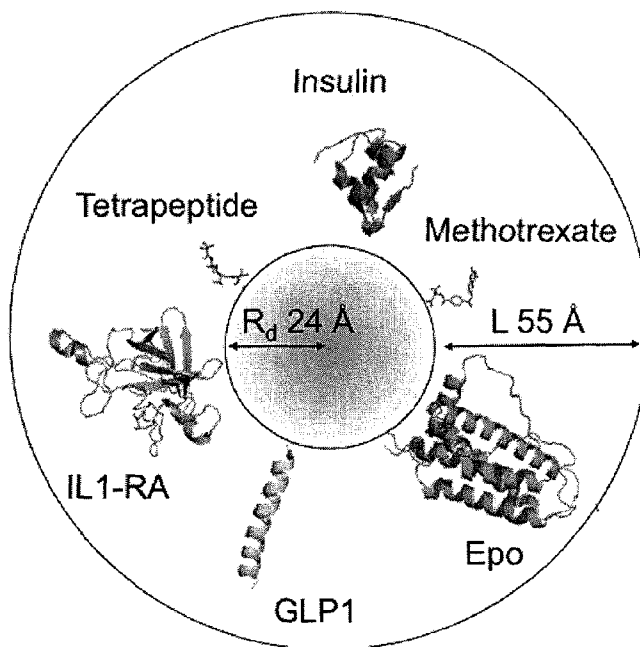
PAMAM 32 -(PEG5000) 30 with therapeutic agents of varying sizes drawn to scale and immersed in the PEG shell. methotrexate (0.454 kDa), insulin (globular, 5.8 kDa), GLP1 ( \alpha -helix, 3.3 kDa), IL1-RA (Anakinra; globular, 17.3 kDa), erythropoietin protein (4-helix bundle, 18 kDa)
