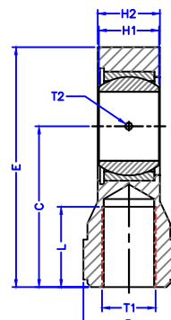
SECTION Z-Z
