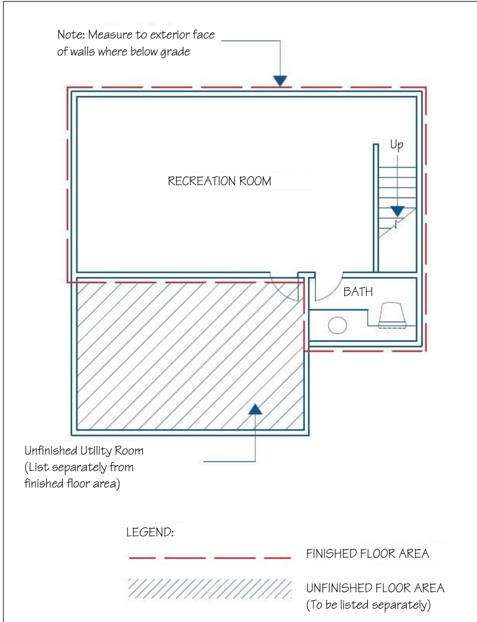
FIGURE 3. Basement Plan (below grade)
