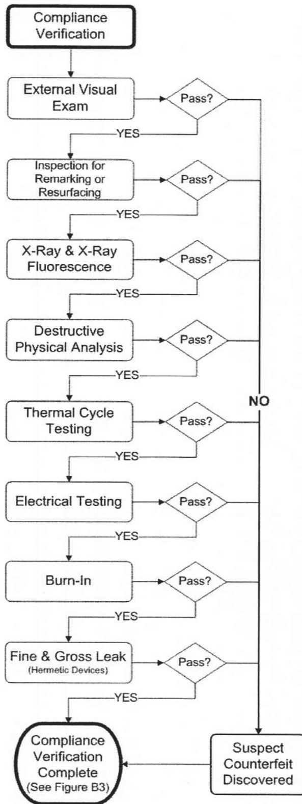
FIGURE E1 - SAMPLE AUTHENTICITY VERIFICATION PROCESS FLOW
