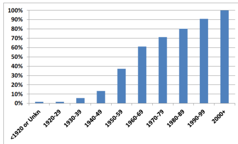
Figure 3. Cumulative Percentage of Pipe Installed by Decade
