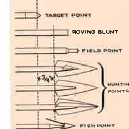
Fig. 2 Arrow Length is Measured from Bottom of Nock to Point Indicated by Dotted Line.
