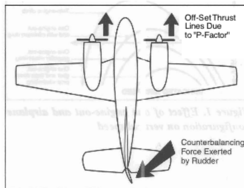
Figure 5. Engine Thrust Line Shifts to Right at Low Airspeeds and at High Angles of Attack
