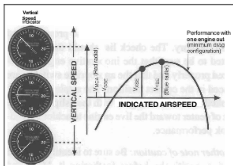
Figure 6. Key Single Engine Airspeeds
