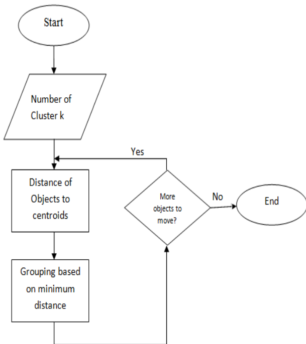
Figure 3: Flowchart of k-means clustering algorithm.
