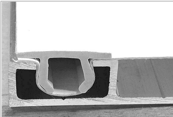
Here the TS79W is inserted in the TS23 extrusion channel.
