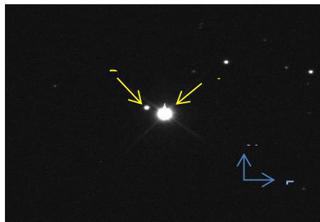
Figure 1. Image from T18 of WDS 03117+8128. Cropped to show target stars.
