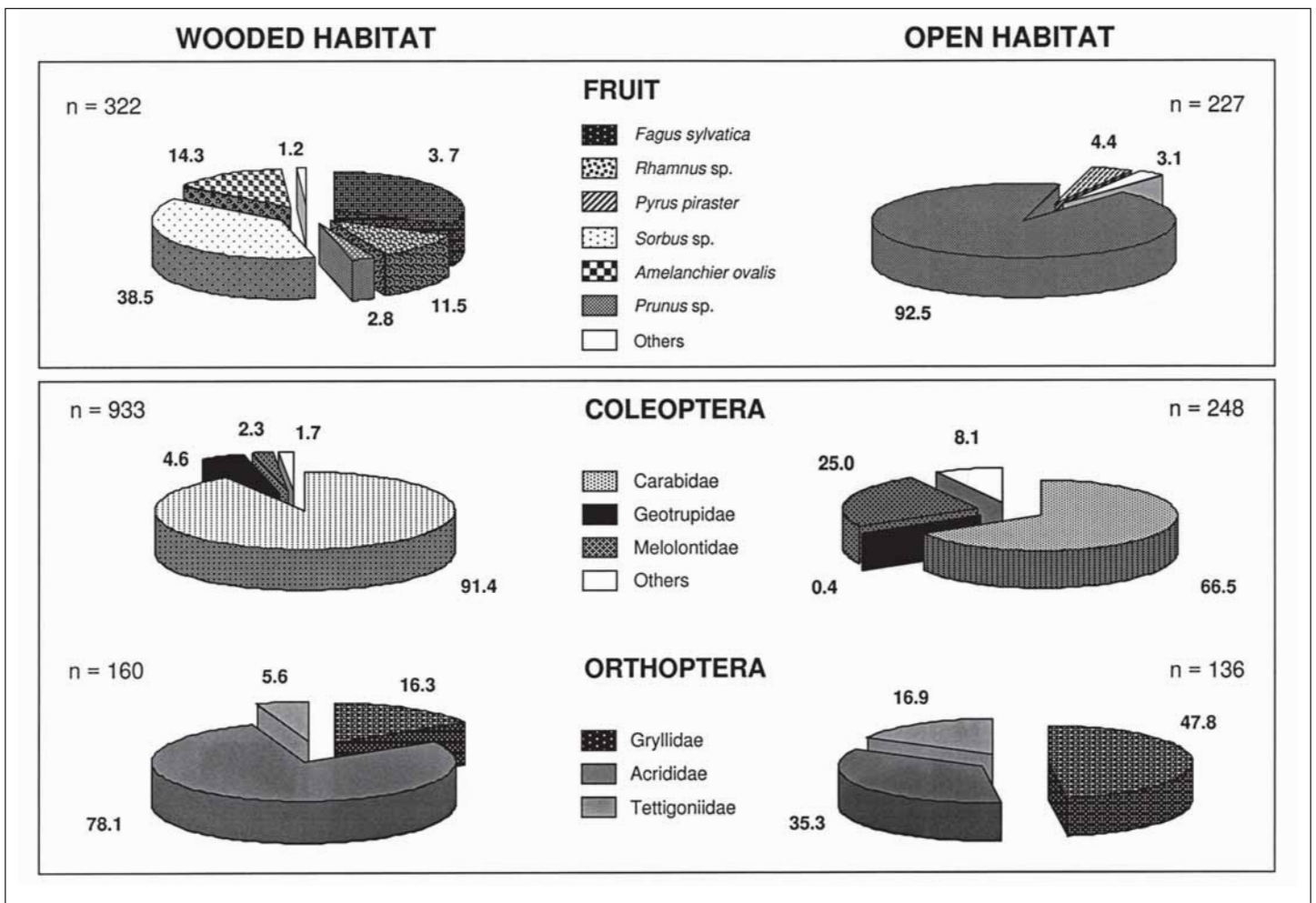
Fig.2. Coleoptera, Orthoptera and fruit composition per habitat in the badger diet in Abruzzo National Park, expressed as relative frequency of occurrence.
