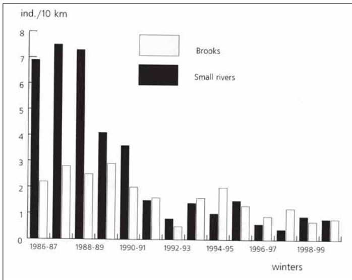
Fig.2. Dynamics of European mink density (ind./10 km water course) in the Lovat river head (winters 1986-2000)
