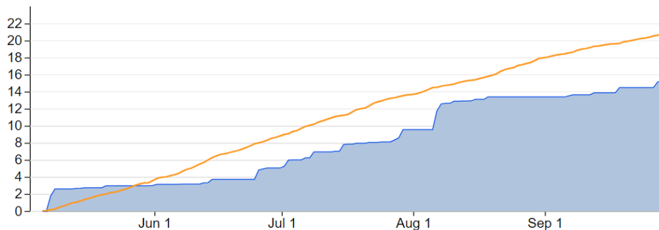
Accumulated Precipitation
