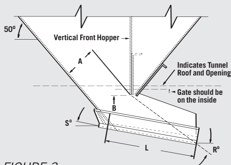
RECOMMENDED HOPPER DESIGN/LENGTH OF DECK IN RELATION TO MATERIAL DEPTH
