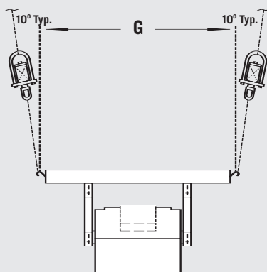
DIMENSIONS (dimensions in inches)
