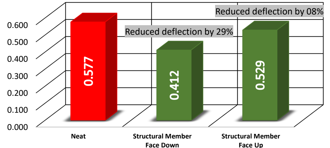
Structural Member- Inches of Deflection
