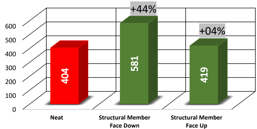
Structural Member-Pounds of Force at Failure
