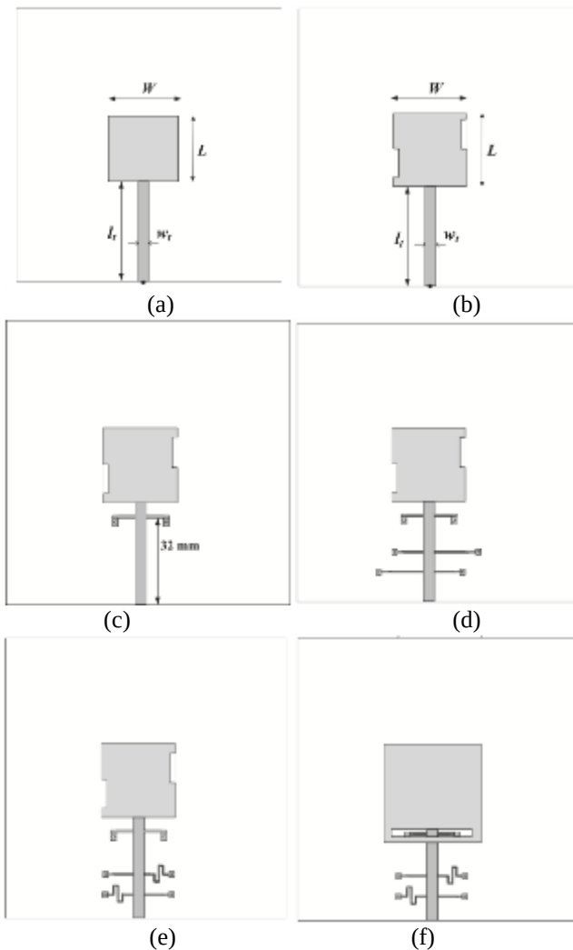
Fig. 2 (a) Basic patch antenna with dimensions ( L = W = 28\text{mm} , l_t = 36\text{mm} and w_t = 2.8\text{mm} ), (b) Improved patch antenna with the asymmetrical cut at left and right edges, (c) Improved patch antenna with shunt inductor at 32mm above from feed point, (d) Improved patch antenna with microstrip resonators, (e) Improved patch antenna with microstrip symmetrical resonators, and (f) Improved patch antenna with parasitic patch and slot.
