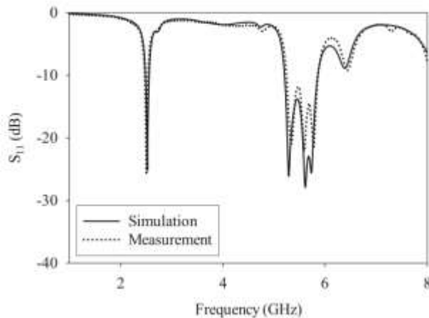
Fig. 1. (g) with harmonic suppression
