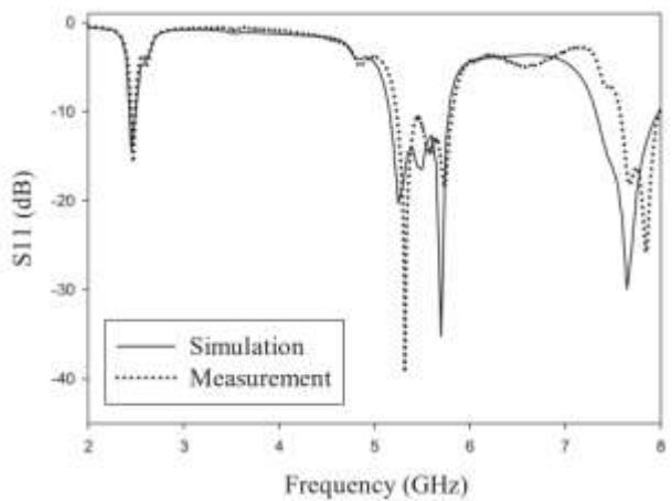
Figure 3. (f) Without harmonic suppression
