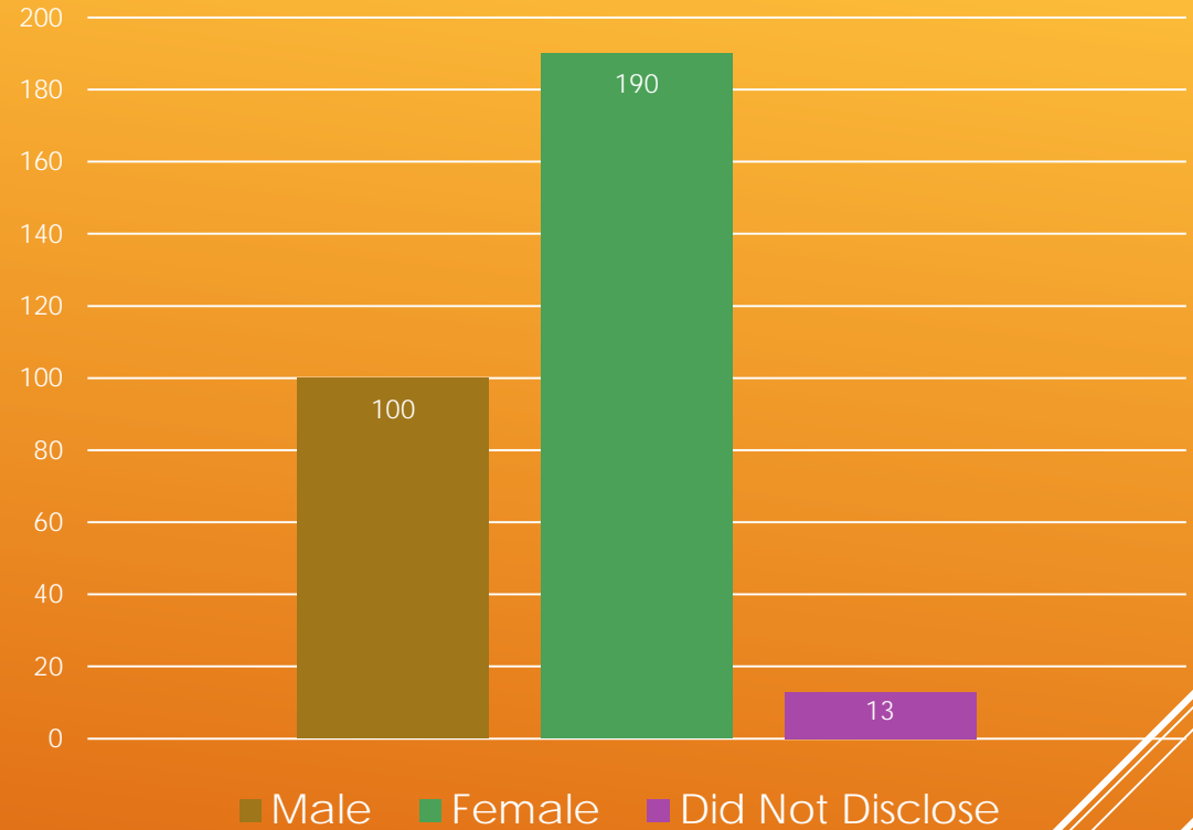
Gender Demographics
