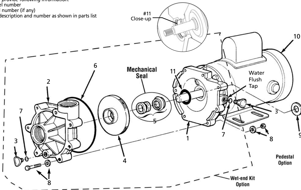
Figure 4 - Repair Parts Illustration
