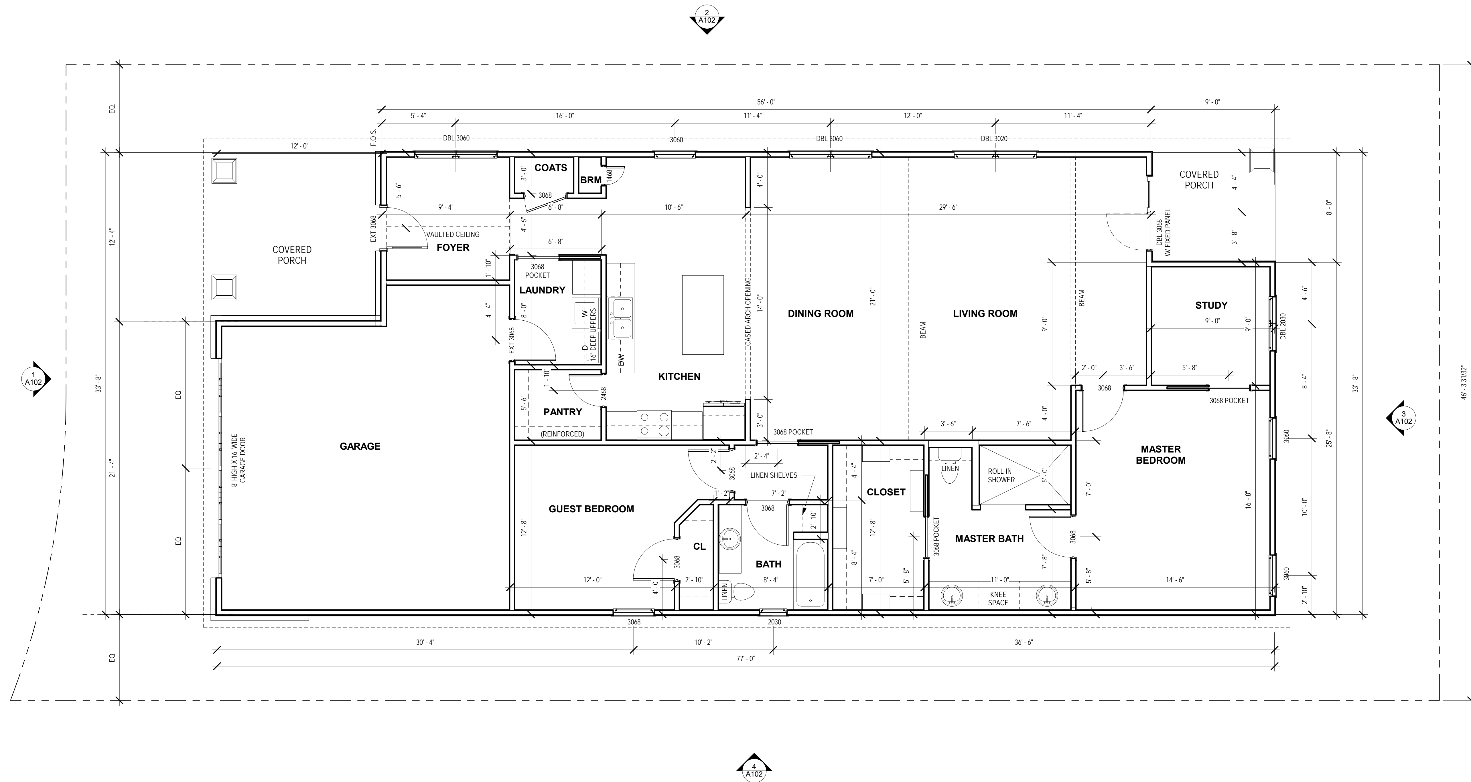
1 FLOOR PLAN 1/4" = 1'-0"
