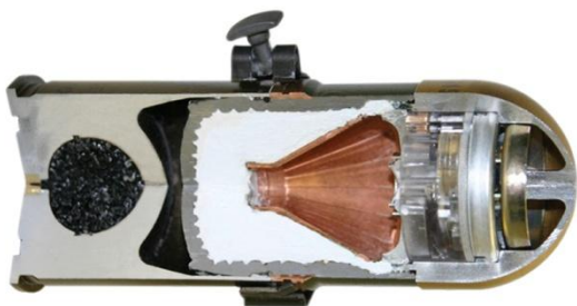
40mm M430A1 HEDP
