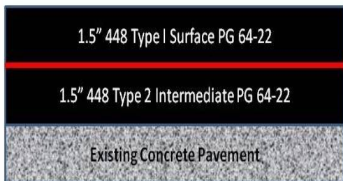
Waterloo Road Cross Section
