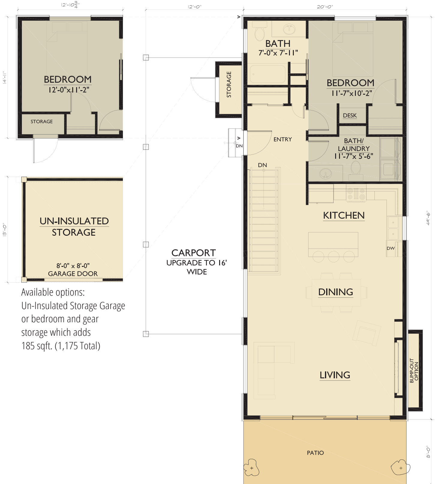
Main Floor Plan 990 sqft
