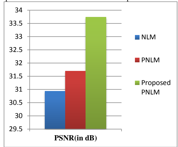
Fig.2: PSNR Comparison
