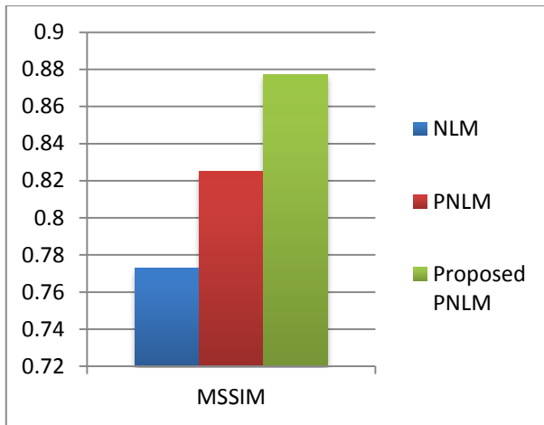
Fig.4: MSSIM Comparison
