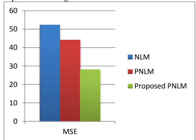
Fig.3: MSE Comparisons
