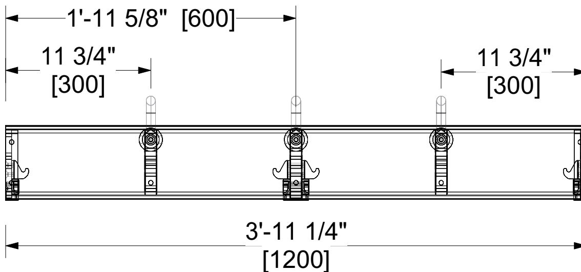
1 Front View 1 1/2" = 1'0"
