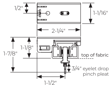
R-TEC Ceiling Mount Bracket RTMDTBCM
