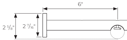
Wall Mount 6" return PTHMT138401
