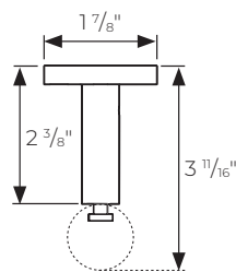
Ceiling Mount Single PTHMT138403
