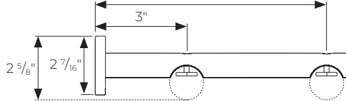
Ceiling Mount Single PTHMT138403
