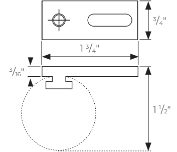
Low-Profile Ceiling Single PTHMT138406
